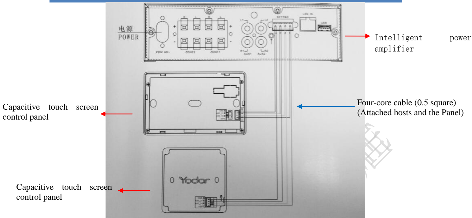
Fig1( CT-ETWF3014-YD Host and Panel wiring diagram)
